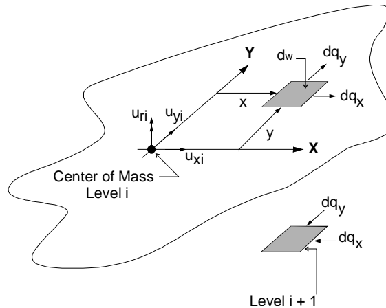
Figure 11.4 Mass Distribution at Typical Floor Level
