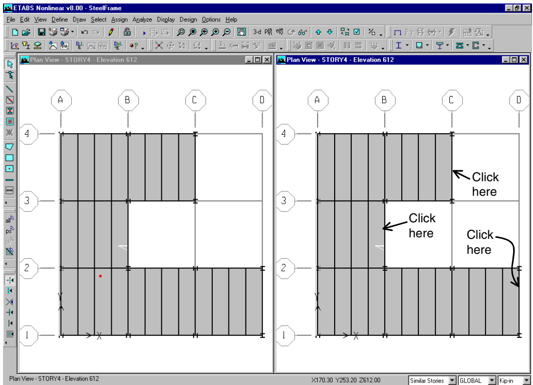
Figure 23 Adding dummy wall-type objects in Plan View
