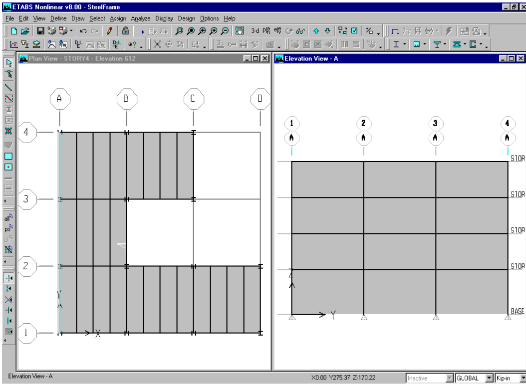
Figure 22 Model in Elevation View after dummy area objects have been added along line A
