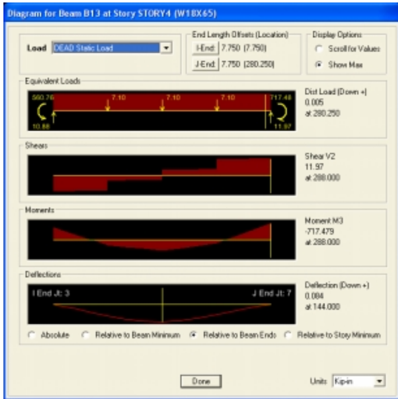
Figure 46 Force details obtained by right-clicking a beam shown in the elevation view in Figure 45
